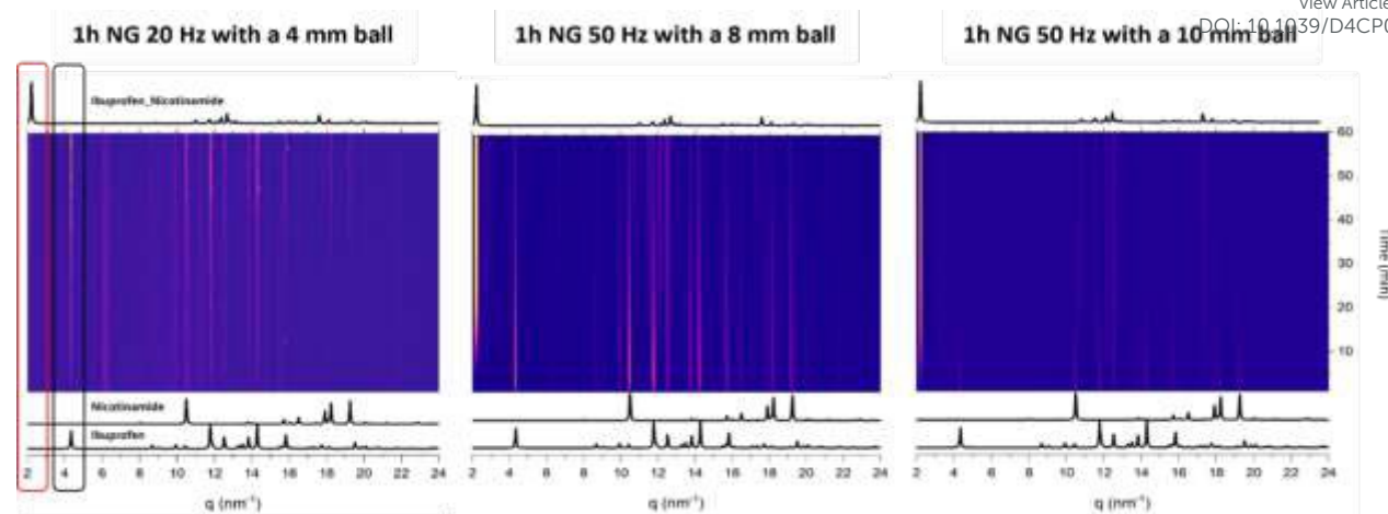
Figure 2. Comparison between the mechanochemical reactions performed at different neat grinding (NG) milling conditions. The black box highlights the disappearance of the reagent peak (ibuprofen), while the red box indicates the emergence of the main co-crystal reflection.
