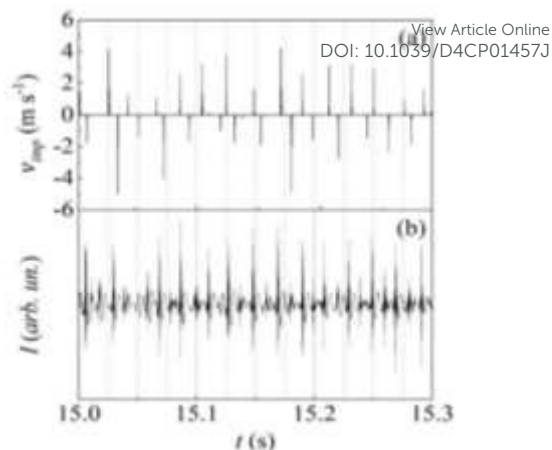
Figure 5. Part of the sequences of impacts obtained from (a) numerical simulation and (b) piezoelectric sensors. Vertical dotted lines are a guide to the eye aimed at facilitating the comparison between the times at which the impacts are detected.
