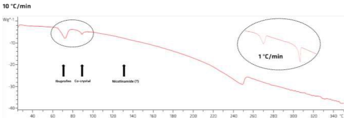
Figure 6. 10°/min DSC trace for the physical mixture ibuprofen-nicotinamide. It is evidenced the melting point of ibuprofen (78 °C), of the co-crystal (90 °C) and the one – missing – of nicotinamide (130 °C). In the black dashed circle on the right, the 1°/min DSC of the physical mixture to better appreciate the formation of the co-crystal among melting.
