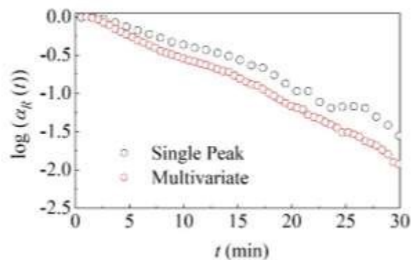
Figure 4. Comparison between single peak (black dots) and MCS-ALS (red dots) analyses in a semi-logarithmic plot for the data collected the first 30 minutes of the reaction.
