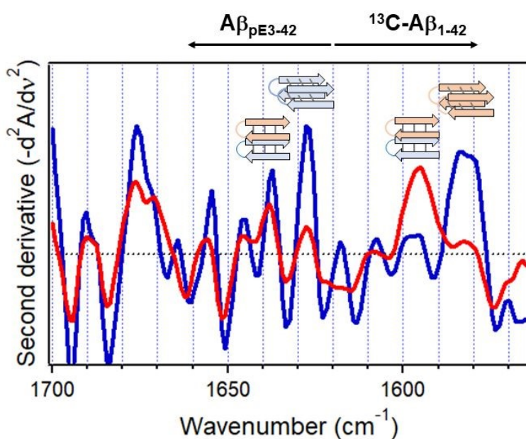
Figure 8. Inverted second derivative amide I spectra of ^{13}\text{C} - \text{A}\beta_{1-42} and \text{A}\beta_{\text{pE}3-42} after 5 h hydration with \text{D}_2\text{O} -saturated nitrogen gas when physically separated (blue) and combined at 1:1 molar ratio (red). Cartoons for homo- or hetero-oligomers stabilized by intermolecular and intramolecular H-bonding, respectively, are shown above respective spectral features ( ^{13}\text{C} - \text{A}\beta_{1-42} , rose, and \text{A}\beta_{\text{pE}3-42} , blue). Reproduced from ref. 37, with permission.
