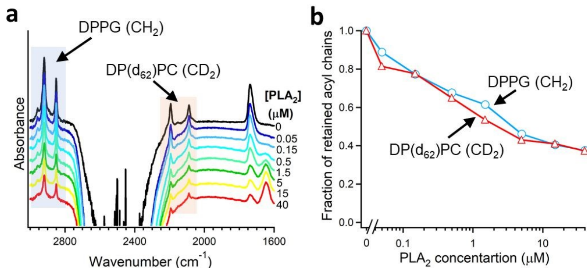
Figure 2. Hydrolysis of the two components of a binary lipid bilayer by \text{PLA}_2 . (a): ATR-FTIR spectra of a lipid bilayer composed of an equimolar combination of DPPG and chain-perdeuterated \text{DP}(d_{62})\text{PC} at different concentrations of \text{PLA}_2 , as indicated. (b): Dependence of the integrated methylene absorbance intensities of both lipids on \text{PLA}_2 concentration. Adapted from ref. 19, with permission.
