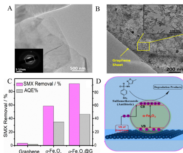
Fig. 11 (A) TEM image of an exfoliated graphene sheet; (B) TEM image of the prepared \alpha-Fe_2O_3@G NCs; (C) photocatalytic antibiotic sulfamethoxazole (SMX) degradation efficiency of graphene, \alpha-Fe_2O_3 , and \alpha-Fe_2O_3@G and their corresponding apparent quantum efficiencies (AQEs) under visible light; and (D) schematic representation showing the possible mechanism for electron transfer for the degradation of SMX antibiotic. Inset of (A) shows the SAED pattern of exfoliated graphene sheets. Adopted from ref. 156 with permission. Copyright 2020 The Royal Society of Chemistry and the Centre National de la Recherche Scientifique.
