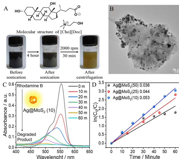
Fig. 14 (A) Molecular structure of [\text{Cho}][\text{Doc}] and exfoliation of \text{MoS}_2 in aqueous [\text{Cho}][\text{Doc}] ; (B) TEM image showing Ag NPs adhered to the \text{MoS}_2 ; (C) time-dependent UV absorbance of RhB in the presence of \text{Ag}@MoS_2(10) under sunlight; and (D) comparison of the kinetics of \text{Ag}@MoS_2(10) NCs, \text{Ag}@MoS_2(25) NCs and \text{Ag}@MoS_2(50) NCs. Adopted from ref. 161 with permission. Copyright 2024 Elsevier B.V.
