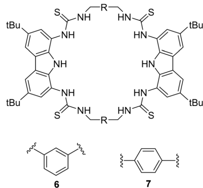
Fig. 4 Chemical structures of macrocycles 6 and 7 . Reported by Jolliffe and colleagues.
