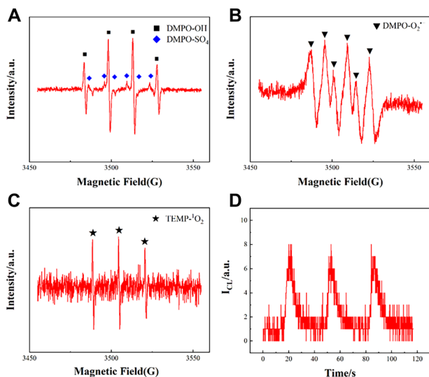
Scheme 2 Schematic representation of the lucigenin-CD CL system in NaOH solution. Reprinted with permission from ref. 52, Copyright 2019 Springer Nature.
