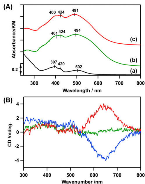
Fig. 1 (A) (a) A transmission UV-vis spectrum of [LCo 3 (NHMe 2 ) 6 ](OTf) 3 in methanol ( c = 0.2 \text{ mol L}^{-1} ). (b) and (c) DR UV-vis spectra of (b) LCo 3 /en-SiO 2 , and (c) LCo 3 ((R)-A1)/en-SiO 2 . (B) DR CD spectra of LCo 3 /en-SiO 2 (green), LCo 3 ((R)-A1)/en-SiO 2 (red) and LCo 3 ((S)-A1)/en-SiO 2 (blue).
