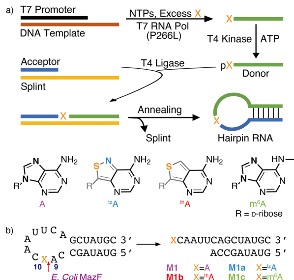
Fig. 1 (a) Enzymatic pathway to site-specifically modified RNAs, replacing an adenosine residue with m^6A , \text{t}^zA , \text{t}^hA . (b) A stem-loop substrate shown to be targeted by E. coli 's MazF. M1 , M1a , M1b , M1c are the native, \text{t}^zA , \text{t}^hA and m^6A modified stem-loop substrate, respectively.
