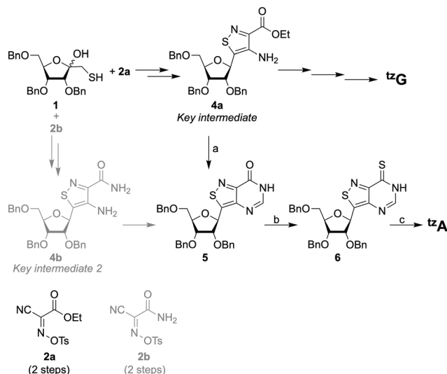
Scheme 1 Previous (gray) and current (black) synthetic pathways to \text{t}^zG and \text{t}^zA , reagents and conditions: (a) formamidine acetate, \text{Et}_3\text{N} , EtOH, reflux, 70%; (b) \text{P}_2\text{S}_5 , pyridine, 90 °C, 2 h; (c) (i) \text{NH}_3 , MeOH, 70 °C, 16 h; (ii) \text{HSCH}_2\text{CH}_2\text{SH} , \text{BF}_3\cdot\text{OEt}_2 , DCM, rt, 72 h, 72% (for steps b and c).
