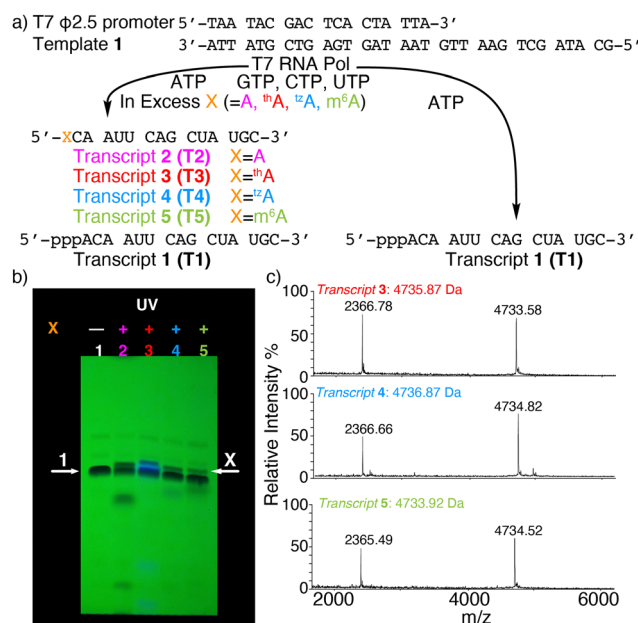
Fig. 2 (a) Transcription reactions in the presence of natural NTPs using the \phi 2.5 T7 promoter and template shown, initiated with large excess (see ESI†) or without X (X = A, \text{t}^hA , \text{t}^zA , or m^6A ). (b) PAGE of transcription reactions using 2.5 mM NTPs with or without modified nucleosides X. Lane 1: native NTPs only. Lane 2: transcription initiation with A (18.75 mM). Lane 3: transcription initiation with \text{t}^hA (18.75 mM). Lane 4: transcription initiation with \text{t}^zA (15 mM). Lane 5: transcription initiation with m^6A (32 mM). White arrows indicate the expected product transcript 1 (arrow 1) and modified transcripts T2 , T3 , T4 , and T5 (arrow X). UV shadowing is done upon illumination at 254 nm; (c) MALDI-TOF MS of transcript T3 , T4 , T5 .
