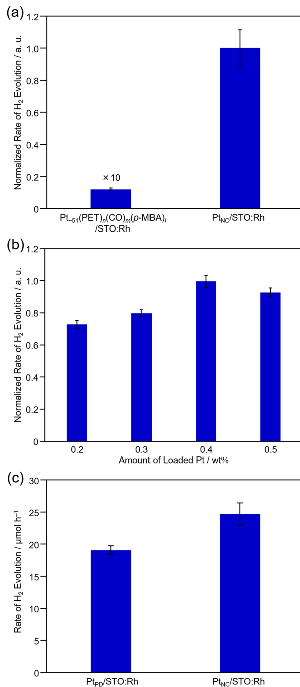
Fig. 5 \text{H}_2 -evolution activity of Pt cocatalyst-loaded STO:Rh photocatalysts. (a) Before ( \text{Pt}_{-51}(\text{PET})_n(\text{CO})_m(p\text{-MBA})_l/\text{STO:Rh} ) and after ( \text{Pt}_{\text{NC}}/\text{STO:Rh} ) calcination of Pt NC-loaded STO:Rh and (b) dependence of loading weight of the Pt cocatalyst for \text{Pt}_{\text{NC}}/\text{STO:Rh} . (c) Comparison of \text{H}_2 -evolution activity between \text{Pt}_{\text{NC}}/\text{STO:Rh} and \text{Pt}_{\text{PD}}/\text{STO:Rh} . In (a) and (c), the loading weight of Pt on them was 0.4 wt%. In order to eliminate the effect of the difference in the activity of each photocatalyst, STO:Rh synthesized in the same batch was used in each experiment (a)–(c).
