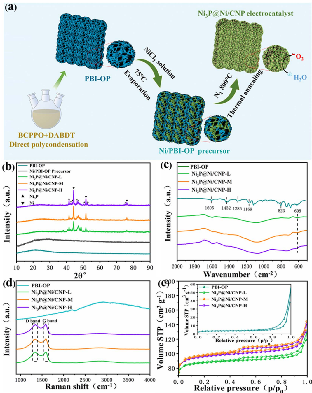
Fig. 2 (a) Schematic illustration of the preparation process of \text{Ni}_3\text{P}@/\text{Ni}/\text{CNP} samples. (b) XRD patterns of PBI-OP, Ni/PBI-OP precursor, \text{Ni}_3\text{P}@/\text{Ni}/\text{CNP} -L, \text{Ni}_3\text{P}@/\text{Ni}/\text{CNP} -M, and \text{Ni}_3\text{P}@/\text{Ni}/\text{CNP} -H. (c) FT-IR spectrum, (d) Raman spectrum, and (e) \text{N}_2 adsorption–desorption isotherms of PBI-OP, \text{Ni}_3\text{P}@/\text{Ni}/\text{CNP} -L, \text{Ni}_3\text{P}@/\text{Ni}/\text{CNP} -M, and \text{Ni}_3\text{P}@/\text{Ni}/\text{CNP} -H.
