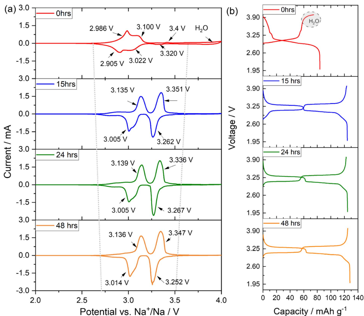
Fig. 7 (a) Selected cyclic voltammety profiles of pristine undried (0 hours) and electrodes dried at 170 °C for 15, 24 and 48 hours under dynamic vacuum at 10^{-2} mbar. Test conducted in three electrode cell using Na metal as counter and reference electrode. Scan rate 0.1 \text{ mV s}^{-1} . (b) First galvanostatic charge/discharge voltage profiles of the same electrodes conducted in coin cell at 0.1C. Both tests are conducted at 25 °C, within the 2.0–4.0 V range. Electrolyte: 1 M NaPF 6 in EC : DEC (3 : 7 v/v%).
