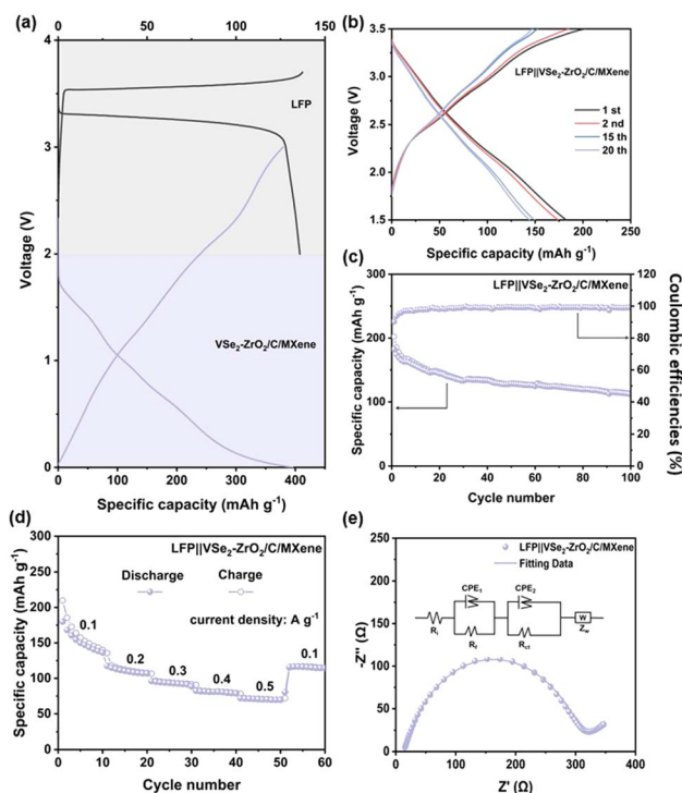
Fig. 8 (a) Half-cell charge–discharge profiles of LFP and VSe 2 -ZrO 2 /C/MXene electrodes at 100 mA g -1 . (b) Galvanostatic charge/discharge profiles and (c) cycling performances for LFP||VSe 2 -ZrO 2 /C/MXene full cell at 100 mA g -1 . (d) Rate performances and (e) Nyquist plot for LFP||VSe 2 -ZrO 2 /C/MXene full cell (inset: equivalent electrical circuit model).
