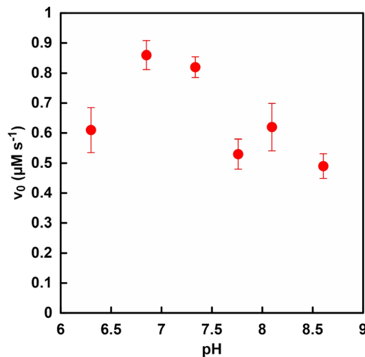
Fig. 2 The pH dependence on the initial rate of fumarate production ( v_0 ) with the system of sodium L-malate and FUM in HEPES buffer with varying pH from 6.3 to 8.6. Each plot shows the mean error of multiple measurements.
