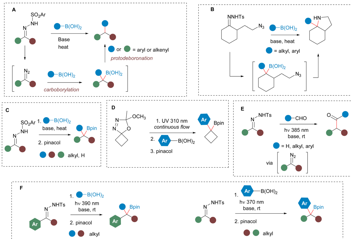
Scheme 1 (A) Reductive coupling of boronic acids and N -sulfonylhydrazones by the carborylation/protodeboronation sequence. (B) Synthesis of pyrrolidines by a C–C/C–N bond forming cascade involving carborylation of a N -tosylhydrazone and intramolecular interception by an azide. (C) Synthesis of pinacol boronates from alkyl N -tosylhydrazones and alkylboronic acids. (D) Synthesis of benzyl boronates by photochemically promoted homologation of arylboronic acids with oxadiazolines. (E) Photoinduced generation of diazo compounds from N -tosylhydrazones and their use in the homologation of aldehydes. (F) This work: synthesis of benzyl boronates by photochemically promoted homologation of alkyl and arylboronic acids with N -sulfonylhydrazones.
