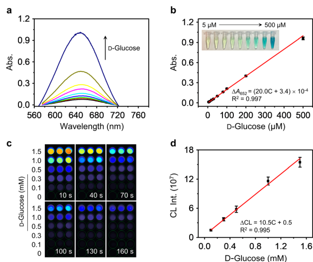
Fig. 5 (a) UV-vis absorption spectra of TMB ( 5.0 \text{ mM} in PBS solution) with increasing D -glucose concentrations ( 5\text{--}500 \mu\text{M} ) catalyzed by AuNPs@PCN-224(Fe) . (b) Plotting the absorption changes of TMB (at 652 \text{ nm} ) as a function of D -glucose concentrations (inset: photo of the TMB/AuNPs@PCN-224(Fe) solutions with different concentrations of D -glucose). (c) Chemiluminescence (CL) imaging of Luminol ( 1 \text{ mM} in PBS solution) with increasing D -glucose concentrations catalyzed by AuNPs@PCN-224(Fe) ( n = 3 ). (d) Plotting the CL intensity changes of Luminol as a function of D -glucose concentrations.
