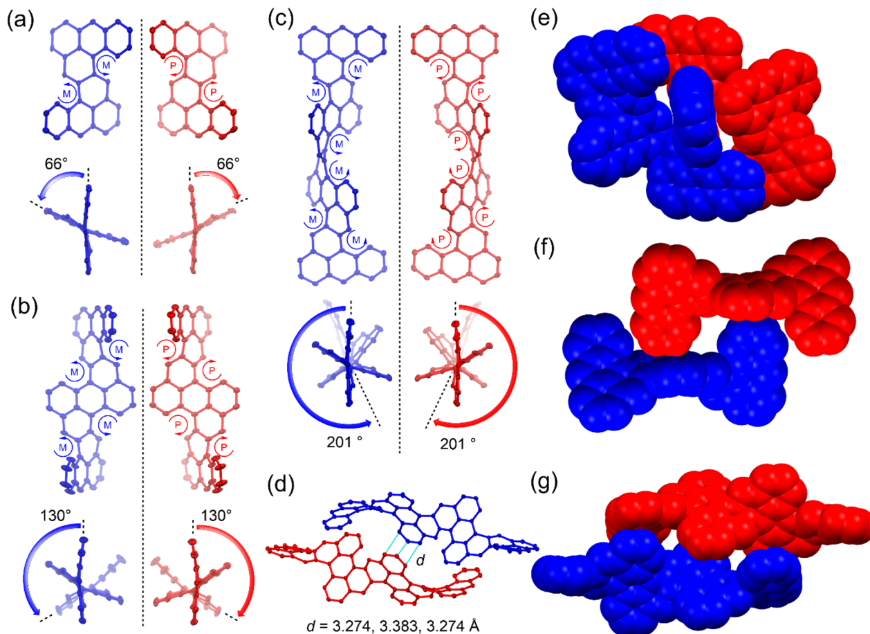
Fig. 2 X-ray crystallographic structures of 1a, 2a and 3b. (a–c) Top view and side view of the crystal structure (backbone only) of 1a, 2a, and 3b, showing 50% probability thermal ellipsoids. (d) Short contacts between the enantiomers of 3b. (e–g) Illustration of the regular packing pattern of 1a, 2a, and 3b.
