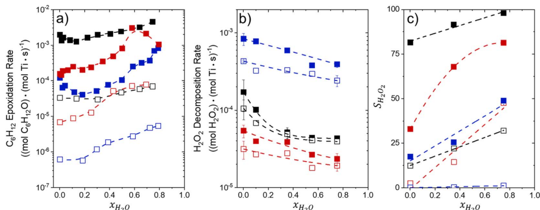
Fig. 1 Turnover rates for (a) \text{C}_6\text{H}_{12} epoxidation to form \text{C}_6\text{H}_{12}\text{O} (1 mM \text{C}_6\text{H}_{12} , 10 mM \text{H}_2\text{O}_2 , 313 K), (b) \text{H}_2\text{O}_2 decomposition (1 mM \text{H}_2\text{O}_2 , 313 K), and (c) \text{H}_2\text{O}_2 selectivities for epoxidation (1 mM \text{C}_6\text{H}_{12} , 10 mM \text{H}_2\text{O}_2 , 313 K) as a function of \text{H}_2\text{O} mole fraction in mixtures of \text{CH}_3\text{CN} (■, □), \text{CH}_3\text{OH} (■, □), and \text{C}_4\text{H}_6\text{O}_2 (■, □) with \text{H}_2\text{O} over Ti-BEA-OH (solid points) and Ti-BEA-F (hollow points). The furthest left data points represent x_{\text{H}_2\text{O}} = 0.002 , which comes from the aqueous \text{H}_2\text{O}_2 reagent solution (39 mM).
