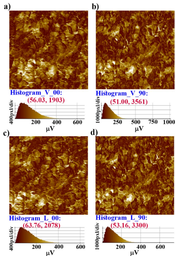
Fig. 4 PFM amplitude image of a crystalline thin film of 1 : (a) and (b) vertical and (c) and (d) lateral amplitude images collected by scanning the X and Y directions; the indication of 0 and 90 is relative. The corresponding histograms show that the maximum number of pixels have the most occurring amplitude value of deformation (in \mu\text{V} ).
