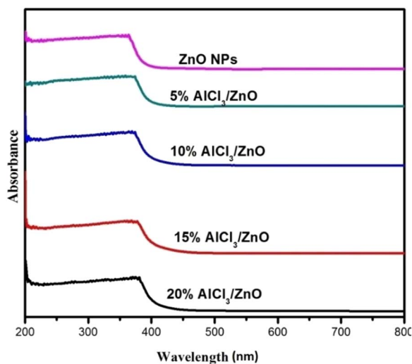
Fig. 5 UV-Vis DRS spectra of as-synthesized pure ZnO NPs, 5% AlCl 3 @ZnO NPs, 10% AlCl 3 @ZnO NPs, 15% AlCl 3 @ZnO NPs and 20% AlCl 3 @ZnO NPs.
