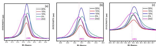
Fig. 4 The shifts in peak position in the X-ray diffraction angles corresponding to (a) (100), (b) (002) and (c) (101) planes for as-synthesized pure ZnO powder and AlCl 3 @ZnO powders corresponding to wt% loadings of 5%, 10%, 15%, and 20%.
