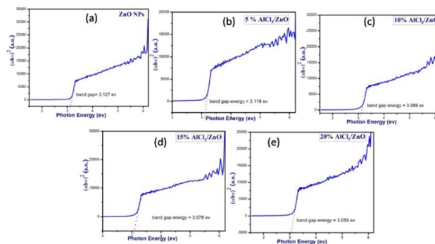
Fig. 6 Tauc plots of (a) as-synthesized pure ZnO NPs and AlCl 3 @ZnO NPs corresponding to wt% loadings of (b) 5%, (c) 10%, (d) 15%, and (e) 20%.
