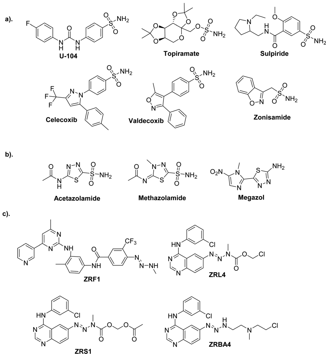
Fig. 1 Commercial drugs on the market contain bioactive cores. (a) Sulfonamides. (b) Thiazolidine sulfonamides. (c) Asymmetrical azines.
