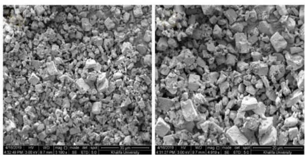
Fig. 23 SEM image zeolite AQSOA-Z02. Reproduced from ref. 88 with permission from Microporous and Mesoporous Materials .
