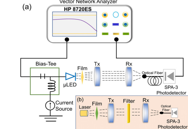
Fig. 3 Bandwidth measurement system architecture for (a) a white light system and (b) color-conversion films.
