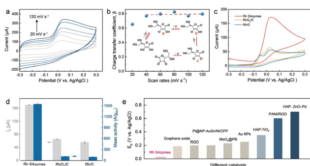
Fig. 2 Electrocatalytic oxidation of AA. (a) CVs of Rh SAzymes in 10 mM AA and 0.1 M PBS at different scan rates (20, 40, 60, 80, 100, and 120 \text{mV s}^{-1} ) and (b) the corresponding \beta versus scan rate. (c) Background-corrected CV curves of Rh SAzymes, RhO x /C, and Rh/C at a scan rate of 50 \text{mV s}^{-1} in 10 mM AA and 0.1 M PBS. (d) The corresponding peak currents and mass activities of Rh SAzymes, RhO x /C, and Rh/C for AA oxidation. (e) Comparison of the anodic peak potential for Rh SAzymes and previously reported catalysts. 42–50
