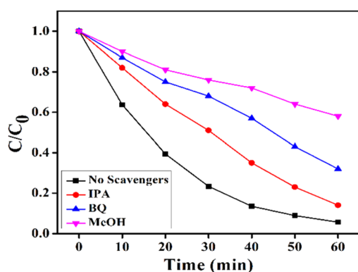
Fig. 14 Photocatalytic degradation of RhB aqueous solution by T-CuS in the presence of IPA, BQ, MeOH and no scavengers.
