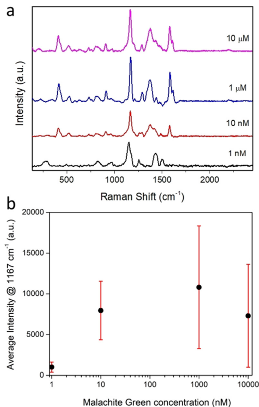
Fig. 6 (a) SERS spectra for CμP-AuNP-1 composite particles incubated with MG at concentrations of 1 nM to 10 \mu M. Spectra shown are from the highest intensity measurement from each MG concentration. Each trace shows an individual particle. (b) Average SERS intensity for the 1167 \text{cm}^{-1} peak as a function of MG incubation concentration. Spectra recorded in \text{H}_2\text{O} with 785 nm excitation.
