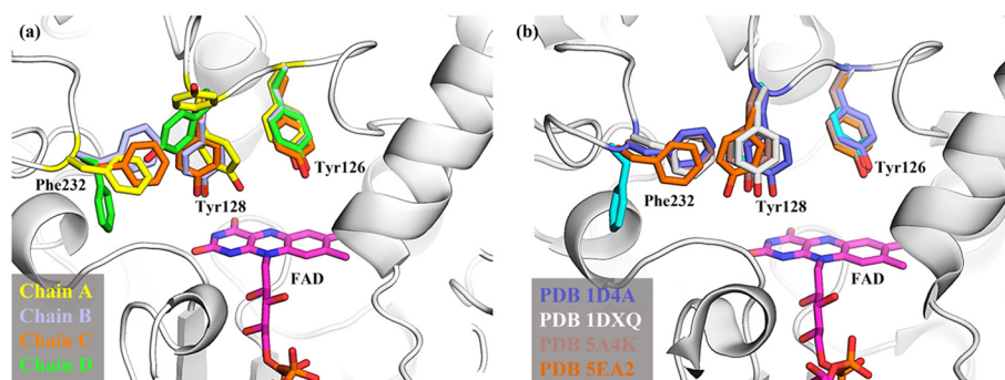
Fig. 7 (a) Superimposition of the four monomers found in the asymmetric unit of the NQO1 structure determined at MFX. Residues Tyr126, Tyr128, and Phe232, key for NQO1 function, are represented as sticks. FAD is labeled accordingly and represented as pink sticks. (b) Superimposition of the four unliganded cryogenic structures of NQO1 (PDB 1D4A, 79 PDB 1DXQ, 79 PDB 5A4K 84 and PDB 5EA2 (ref. 85)). As in (a), the key residues and FAD molecule are highlighted.
