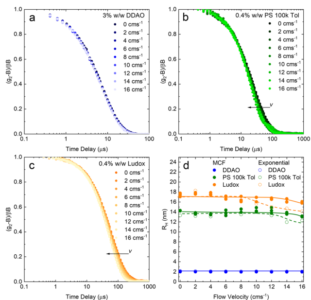
Fig. 7 (a) DLS correlograms obtained for a solution of 3% w/w DDAO in water as a function of flow velocity ( 0\text{--}16\text{ cm s}^{-1} ) in a 1 mm ID glass capillary. (b) idem for 0.4% w/w PS 100k in toluene, (c) idem for 0.4% w/w Ludox AS 40 in water. (d) Apparent R_H extracted from the velocity-dependent model (solid lines and symbols); for comparison, results from a simple exponential decay (dashed lines and open symbols) are included.
