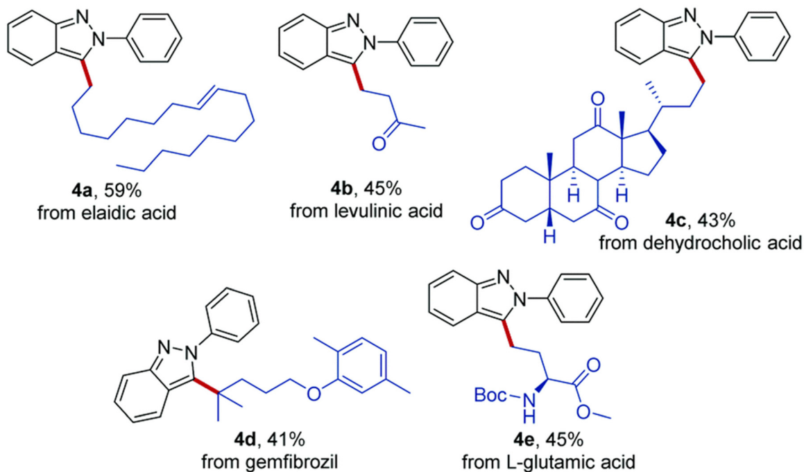
Scheme 11 Late-stage modification of natural resources and drug molecules. Reaction conditions: 1a (0.2 mmol), 2 (2 equiv.), 4CzIPN (5 mol%), DABCO (1 equiv.), DMC (2 mL), T = 35\text{ }^\circ\text{C} , blue LED, t = 12\text{ h} under N_2 atmosphere. Reproduced with permission from ref. 108. Copyright 2021 Chinese Chemical Society (CCS), Shanghai Institute of Organic Chemistry (SIOC), and the Royal Society of Chemistry.
