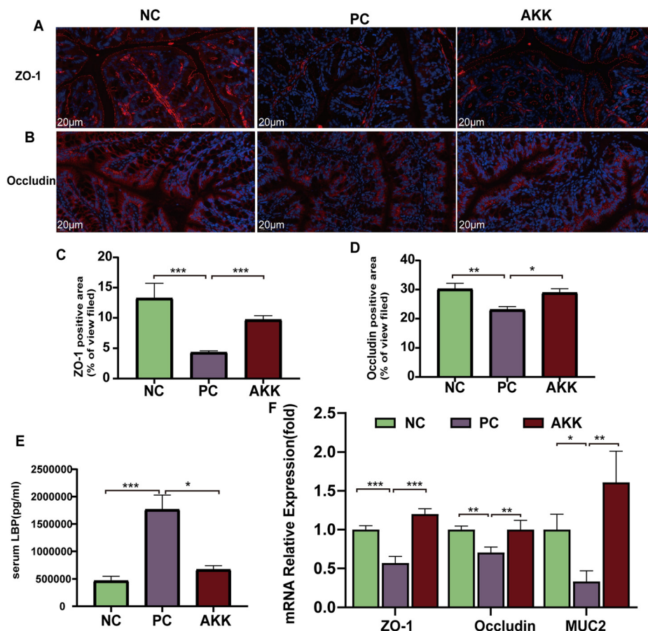
Fig. 3 A. muciniphila improved gut barrier function and inhibited lipopolysaccharide stimulation. Representative images of ZO-1 (A) and occludin (B) immunohistochemical staining (scale = 20 \mu m). By using ImageJ, the percentage of positive area (ZO-1 and occludin, respectively) was calculated; n = 3 per group and five randomly selected visual fields (C and D). Serum LBP (E) levels were measured by ELISA ( n = 8 each group). (F) The mRNA expression levels of ZO-1, occludin, and MUC2 were normalized to Gapdh mRNA levels ( n = 8 each group). Data are shown as the mean \pm standard error of the mean (mean \pm SEM); compared with the PC group, * p < 0.05 , ** p < 0.01 , and *** p < 0.001 . NC, PBS + saline group; PC, PBS + LPS group; AKK, A. muciniphila + LPS group.
