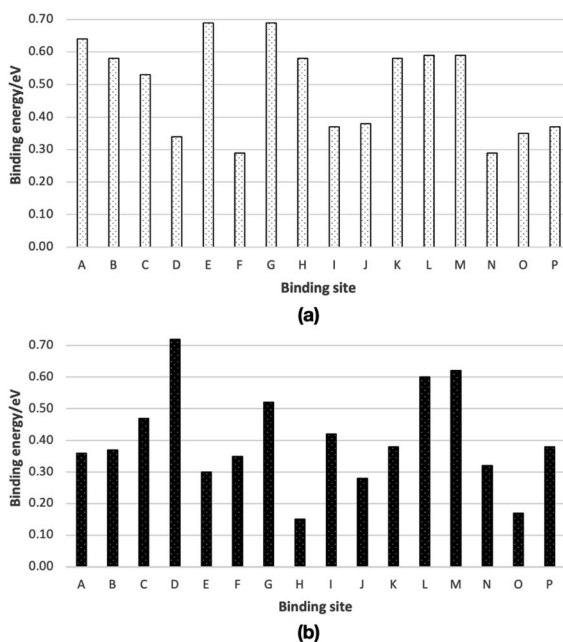
Fig. 3 Calculated binding energies of (a) a \text{CH}_2\text{OH} radical and (b) a \text{CH}_3\text{OH} on ice, from ONIOM( \omega\text{B97X-D/Def2-TZVP:AMOEBA09} ) calculations. Optimized molecular structures are shown in Fig. S1 and S2.† Binding energies are summarized in Table S1.†
