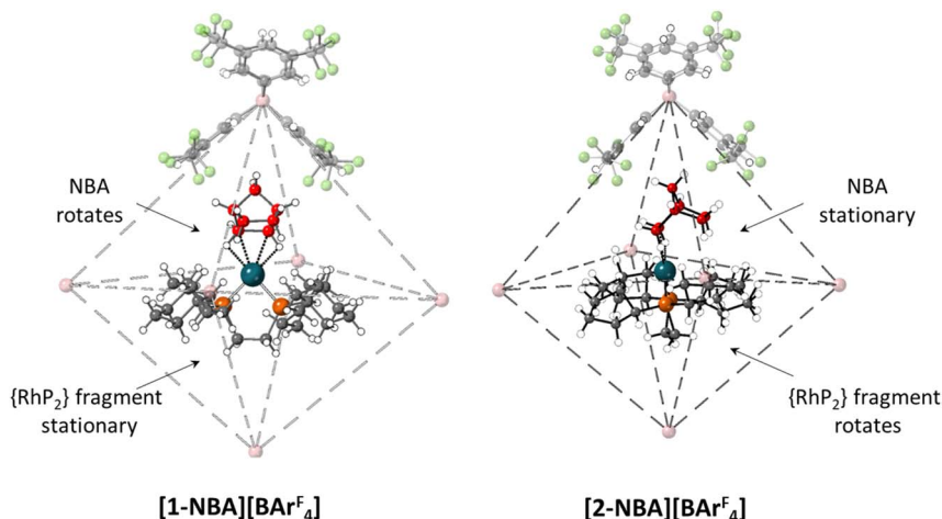
Fig. 10 Packing diagrams contrasting the relative orientations of the NBA and {RhP 2 } fragments in [1\text{-NBA}][\text{BARF}_4] and [2\text{-NBA}][\text{BARF}_4] . The top anion is shown in full along with the B atoms of the other anions within the octahedral array. Carbon atoms of the \sigma -alkane ligands are highlighted in red.
