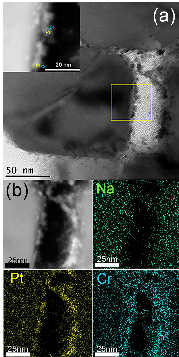
Fig. 7 (a) TEM and ADF-STEM (inset) images and (b) ADF-STEM image along with STEM-EDS elemental maps of the cross-section of a 0.9 wt% \text{Cr}_2\text{O}_3/0.23 \text{ wt% Na } 0.3 \text{ wt% Pt/BaTaO}_2\text{N:Zr0.01} sample.
