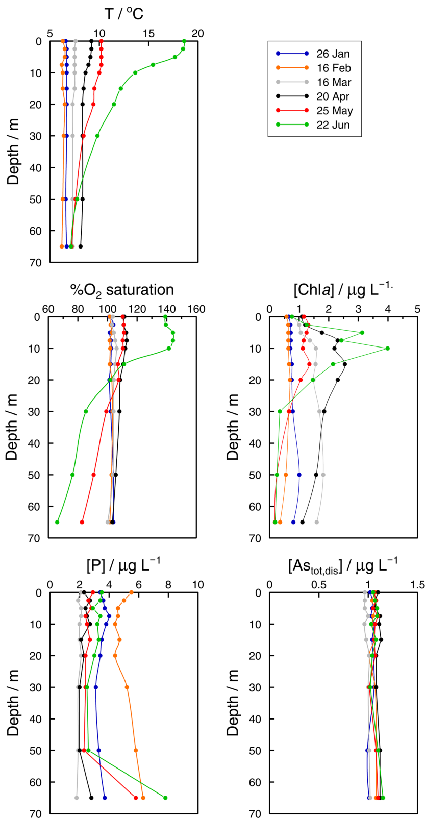
Fig. 3 Vertical profiles of temperature, percentage of \text{O}_2 saturation, chlorophyll a, dissolved reactive phosphorus (DRP), and total 'dissolved' arsenic, \text{As}_{\text{total,dis}} , concentrations in the Petit Lac (point GE3) from January to June 2021.
