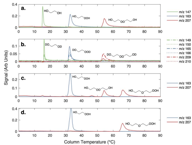
Fig. 2 (a) GC traces of three products of the ethene oxidation experiments: ethylene glycol ( m/z 147), accretion product ( m/z 207), and ROOH ( m/z 163). (b) GC traces with D_2O added to flow tube. Dashed lines are signals at m/z + 2 for each product shown in a, and dotted lines are the signals at m/z + 3 for each product. Solid lines are signals at each original product m/z . (c) GC traces of m/z 163 and m/z 207 from the synthesized standard prior to prep TLC purification. (d) GC traces of m/z 163 and m/z 207 from the standard after purification by preparatory TLC.
