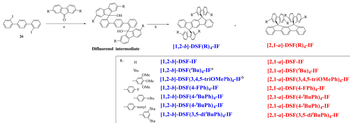
Scheme 19 Synthesis of [1,2- b ]-DSF(R) 4 -IF and [2,1- a ]-DSF(R) 4 -IF. (a) t BuLi, THF, −78 °C to RT, (b) CH 3 CO 2 H/HCl, 100 °C ( a : named [1,2- b ]-7 in Scheme 4, b : named [1,2- b ]-9 in Scheme 4).
