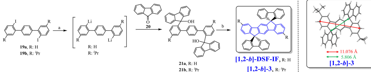
Scheme 6 Left: Synthesis of [1,2- b ]-DSF-IF and [1,2- b ]-3 . 69 BuLi, THF, -78 °C. (b) AcOH/HCl reflux. Right: X-Ray structure of [1,2- b ]-3 .
