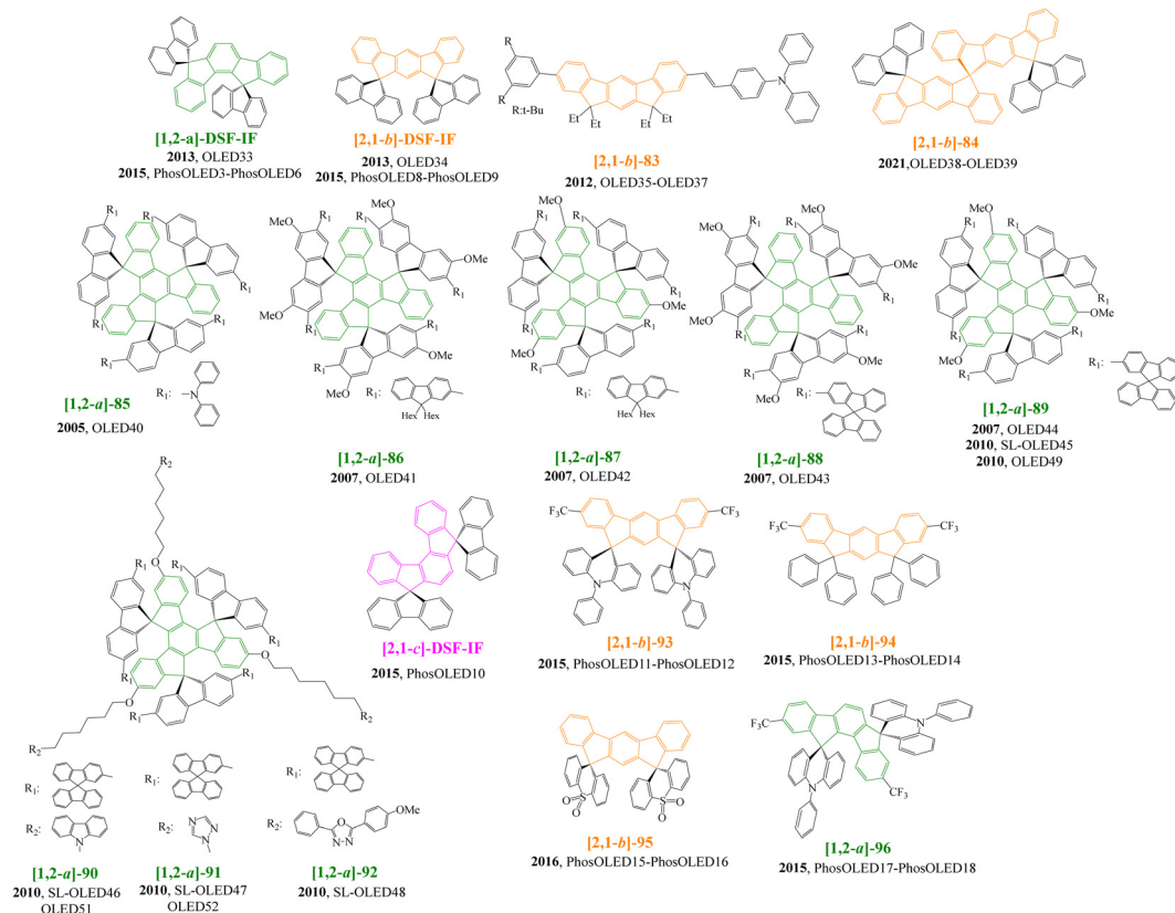
Scheme 24 Molecular structure of organic semiconductors based on [2,1-b]-, [1,2-a]- or [2,1-c]-indeno[1,2-b]fluorenyl cores used in OLED or PhOLEDs.
