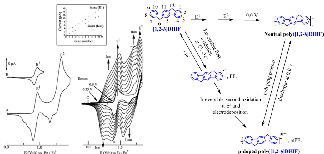
Fig. 3 Cyclic voltammetry in the presence of [1,2- b ]DHIF ( 2 \times 10^{-3} \text{ M} ) (A–C) in \text{CH}_2\text{Cl}_2 ( \text{Bu}_4\text{NPF}_6 0.2 M); working electrode: Pt disk diameter 1 mm; sweep-rate 100 \text{ mV s}^{-1} . The potential limit was of 0.0 to 1.75 V in A; 0.0 to 1.0 V in B; –0.2 to 1.73 V in C. The current scale S is equal to 2 in (A) and to 4 in (B) and in (C). The inset reports the I_{\text{max}} at E 1 and -I_{\text{max}} at I cat vs. the scan number. Adapted from ref. 48 with permission from the Royal Society of Chemistry.
