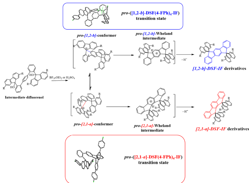
Fig. 8 Middle: Cyclization reaction of difluoreneols with the corresponding intermediates hypothesized. 143 Top and Bottom: Modelization of pro -[1,2- b ]-DSF(4-FPh) 4 -IF and pro -[2,1- a ]-DSF(4-FPh) 4 -IF transition states 144 showing the postulated steric hindrance at the origin of the selectivity observed.
