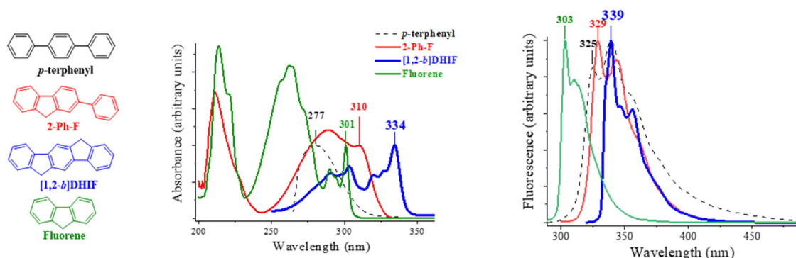
Fig. 2 Absorption (left) and emission (right) spectra of [1,2- b ]DHIF (absorption/emission recorded in \text{CH}_2\text{Cl}_2/\text{decane} ) and of model compounds p -terphenyl, 2-Ph-F and fluorene (all recorded in cyclohexane).
