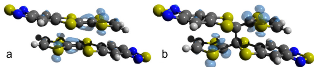
Fig. 7 Fukui function f^{(0)}(r) for (\text{TTF-BTD})_2 radicals before and after the addition reaction. (a) f^{(0)}(r) for the non-covalent \pi -pair “extracted” from the crystal structure at 40 GPa. (b) f^{(0)}(r) for the covalent \sigma -dimer extracted from the crystal structure at 50 GPa. Graphic elaboration performed with isovalue = 0.003 a.u. in Avogadro. 64
