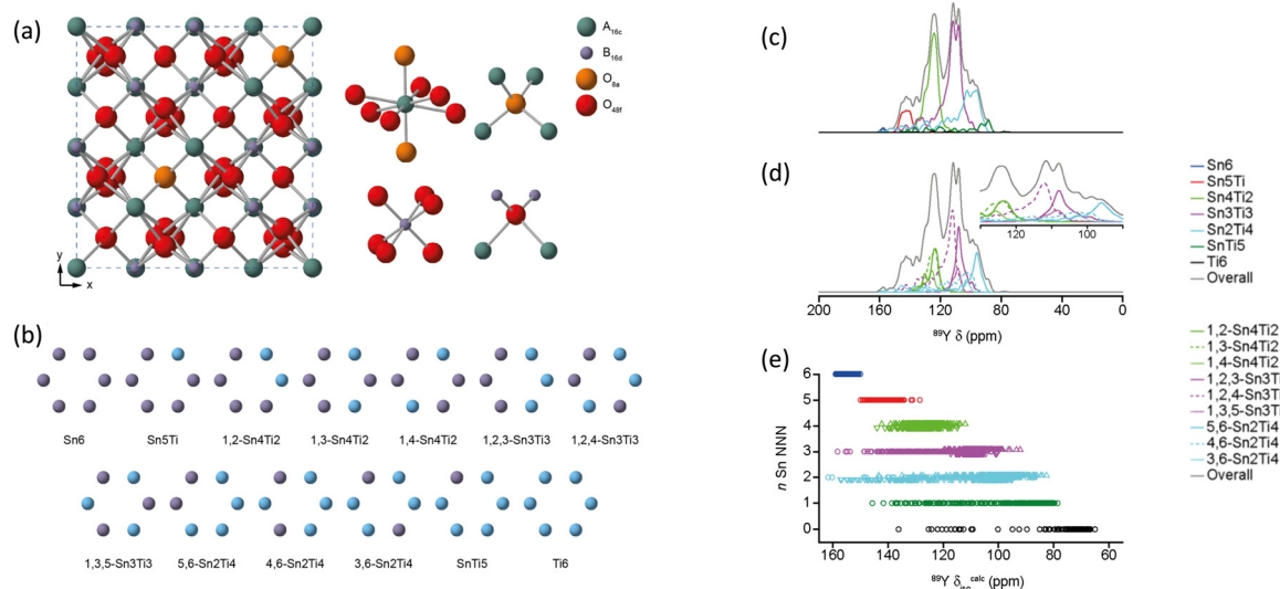
Fig. 7 (a) Structure of a typical \text{A}_2\text{B}_2\text{O}_7 pyrochlore, with expansions of the local environments of the Wyckoff 16c (A), 16d (B), and 8a and 48f(O) sites. (b) Possible arrangements on the six NNN B sites that surround the pyrochlore A and B sites for \text{Y}_2(\text{Sn},\text{Ti})_2\text{O}_7 . (c) ^{89}\text{Y} MAS NMR spectra of \text{Y}_2\text{SnTiO}_7 showing the breakdown into different components assuming full tin/titanium disorder, with the isotropic chemical shift decreasing as the number of NNN tins decreases. (d) The fine detail is produced when the different ordering of the tin/titanium for a given number of NNN tin is also considered. (e) The DFT calculated shift ranges show significant overlaps of different NNN tins across the structural models generated. 88 Reproduced from ref. 88 with permission from the American Chemical Society, copyright 2019.
