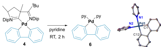
Fig. 2 Solid state structures for the di(pyridine) complexes 6 . Thermal ellipsoids at 50% probability. Hydrogen atoms and co-crystallized solvent molecules are omitted for clarity. Selected bond lengths [Å]: Pd1–N1, 2.127(3); Pd1–N2, 2.128(3); Pd1–C1, 2.002(3); Pd1–C12, 2.002(3).
