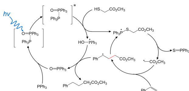
Fig. 2 Plausible mechanism for TPPO-TPP enabled C–C coupling via de-S.
