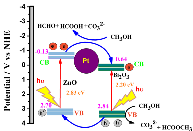
Fig. 12 Schematic mechanism of methanol photo-oxidation by Pt-ZnO-Bi 2 O 3 ternary catalyst.
