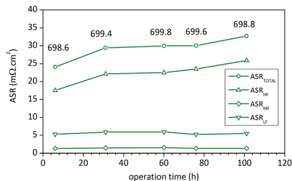
Fig. 7 Long-term operation test of LSC75–GD MW 25 cathode at 700 °C during 101 h under synthetic air flow. The evolution of each component with time shows the origin of the increment in ASR TOTAL observed during the first hours of operation. The inserted numbers indicate the temperature of the sample in °C when the measurement was performed.
