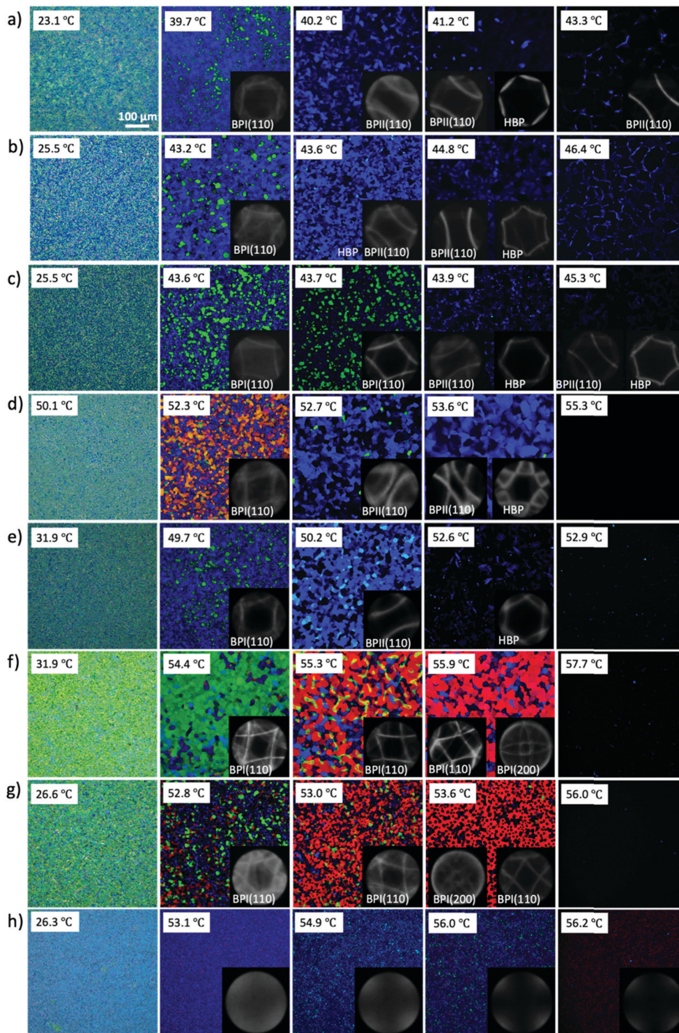
Fig. 2 Hybrid confinement of different RM82 concentrations in the BP premixture: (a) 4.0 wt%, (b) 5.6 wt%, (c) 7.6 wt%, (d) 9.6 wt%, (e) 13.0 wt%, (f) 15.0 wt%, (g) 17.0 wt%, (h) 20.0 wt%. Scale bar: 100 \mu\text{m} .
