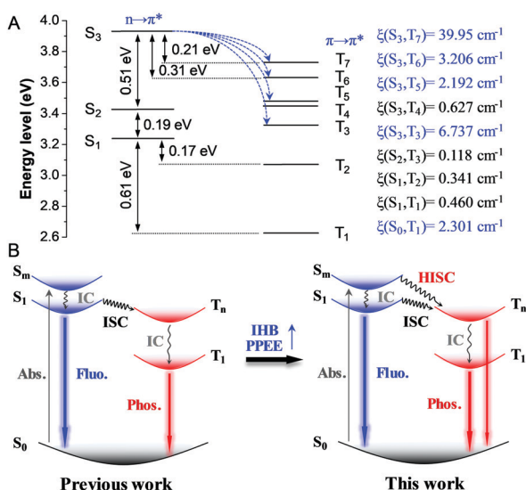
Fig. 3 (A) Schematic diagrams of the TD-DFT calculated energy levels, possible HISC channels and spin-orbit coupling matrix elements of CzPMBBr. (B) Proposed mechanism of UORTP produced by the high-lying intersystem crossing between S_m ( m > 1 ) and T_n ( n > 1 ). ( S_0 = ground state, S_1 and S_m = excited singlet state, T_1 and T_n = excited triplet state, Abs. = Absorption, Fluo. = Fluorescence, Phos. = Phosphorescence, ISC = intersystem crossing, IC = internal conversion, HISC = the intersystem crossing between high-lying S_m ( m > 1 ) and T_n ( n > 1 ), IHB = intra-molecular hydrogen bonding, PPEE = push-pull electron effect)
