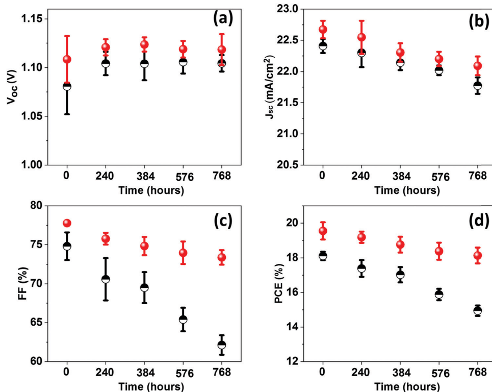
Fig. 5 The photovoltaic parameters ( V_{oc} , J_{sc} , FF and PCE ) of the pristine (black colour) and 5\text{ mg mL}^{-1} CBSC passivated perovskite solar cells (red colour) for the duration of 768 hours in the dried box.
