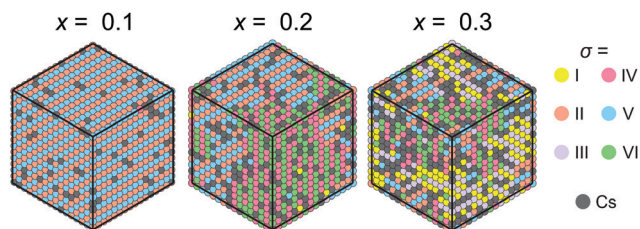
Fig. 7 Snapshots of simulations of our model for different Cs + ion concentrations. The FA cation states are represented in the \sigma -representations. Simulations are performed starting from the disordered phase and gradually lowering the temperature significantly below T_0 . A multidomain structure is observed at the higher mixing levels. Simulation parameters: \epsilon_1 = 21 meV, \epsilon_2 = 12.6 meV, \epsilon_{\text{CS}} = 31.5 meV, L = 16 .
