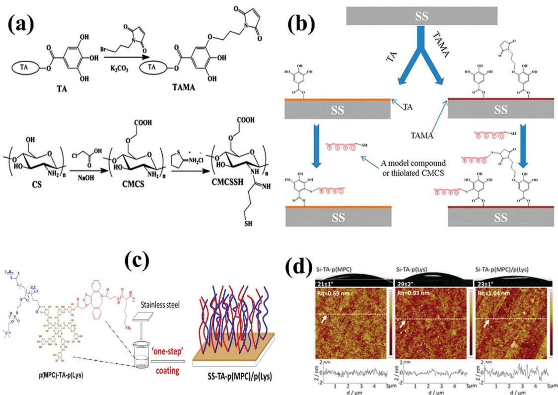
Fig. 5 (a) Synthesis of TAMA and CMCSH. (b) Schematic of the TAMA preparation and anchoring on SS surface via bioinspired approach and subsequent functionalization with thiol-containing compounds via Michael addition (reprinted with permission from ref. 44. Copyright © 2016, American Chemical Society). (c) Schematic illustration of "One-Step" SS surface modification using TA-scaffolded polymer brush. (d) WCA photographs and AFM topography with cross-sectional height profiles of the Si-TA-p(Lys), Si-TA-p(MPC), and Si-TA-p(MPC)/p(Lys) surfaces (reprinted with permission from ref. 98. Copyright © 2019, American Chemical Society).
