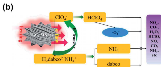
Fig. 12 The roles of active sites. (a) The DBT activation process under the action of \cdot O_2^- and \cdot OH radicals. Reproduced with permission. 44 Copyright 2020, Elsevier. (b) The thermal decomposition of DAP-4 with the assistance of \cdot O_2^- . Reproduced with permission. 128 Copyright 2020, Elsevier. (c) The reaction pathway and important structures of ethylbenzene dehydrogenation on Ti_3C_2O_2 . Ti is shown in light gray, C in dark gray, O in red, and H in white. Reproduced with permission. 95 Copyright 2018, American Chemical Society.
