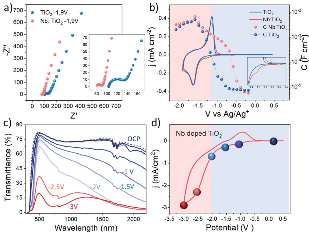
Fig. 5 (a) Nyquist Plot of bare and Nb doped \text{TiO}_2 at -1.9\text{ V vs. Ag/Ag}^+ . (b) Cyclic voltammetry (solid lines) and charge capacitance (balls) associated with the different potential points of \text{TiO}_2 (blue) and Nb-doped \text{TiO}_2 (red). (c) Transmittance spectra and (d) cyclic voltammogram of a lab-scale device of Nb doped \text{TiO}_2 at 50\text{ mV s}^{-1} . The spheres represent the potential points at which the transmittance measurements of the device have been carried out.
