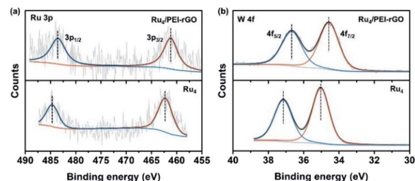
Fig. 4 The high-resolution (a) Ru 3p and (b) W 4f XPS spectra of \text{Ru}_4 and \text{Ru}_4/\text{PEI-rGO} .
