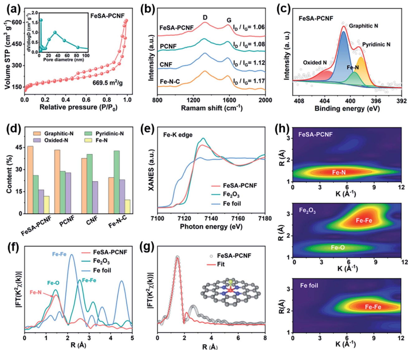
Fig. 2 (a) \text{N}_2 adsorption–desorption isotherms of FeSA-PCNF. The inset shows the corresponding pore size distribution curve. (b) Raman spectra of FeSA-PCNF, PCNF, CNF and Fe–N–C. (c) N 1s XPS of FeSA-PCNF. (d) The relative ratios of different N species in different samples. (e) Fe K-edge XANES spectra of FeSA-PCNF, \text{Fe}_2\text{O}_3 , and Fe foil. (f) Fe K-edge FT-EXAFS spectra of different samples and the corresponding fitting curve of FeSA-PCNF. The inset shows the model of the proposed \text{FeN}_4 structure. The blue, gray, red, and green balls indicate N, C, Fe, and O atoms, respectively. (g) Fe K-edge FT-EXAFS spectra of FeSA-PCNF and the corresponding fitting curve of FeSA-PCNF. The inset shows the model of the proposed \text{FeN}_4 structure. The blue, gray, red, and green balls indicate N, C, Fe, and O atoms, respectively. (h) Wavelet transform plots of FeSA-PCNF, \text{Fe}_2\text{O}_3 , and Fe foil.
