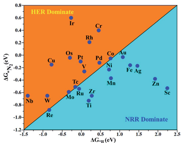
Fig. 4 Calculated Gibbs free energies of \text{N}_2 and \text{H}_2 adsorbed on the M_1 /PMA cluster, which are divided into the eNRR region ( \Delta G_{\text{H}^*} > \Delta G_{^*\text{N}_2} ) and HER region ( \Delta G_{\text{H}^*} < \Delta G_{^*\text{N}_2} ).
